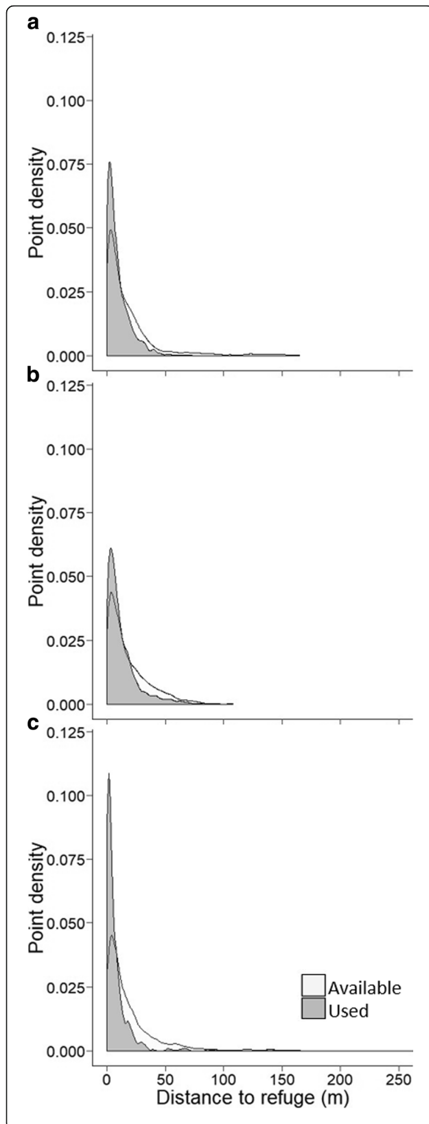
Fig. 3 Density plots of GPS logged points from Callospermophilus lateralis depicting distance traveled from the refuge (m) during two seasons of food availability: a ) Bitterbrush and b ) Interval (no seed available), and c ) Pine. The dark gray indicates used points (gained from GPS loggers) and the light gray indicates randomly generated available points. Study was conducted July 15–September 30, 2014, in the Whittell Forest and Wildlife Area, NV, USA
