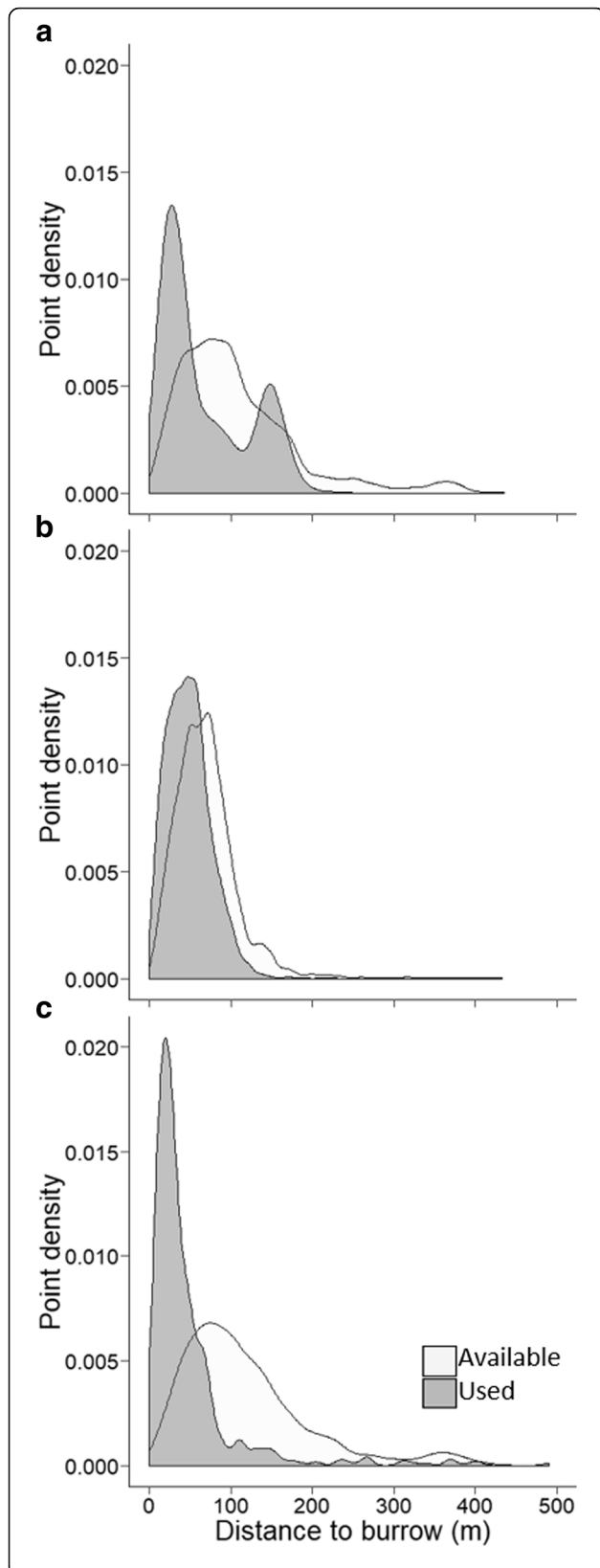
Fig. 2 Density plots of GPS logged points from Callospermophilus lateralis depicting distance traveled from the burrow (m) during three seasons of food availability: a ) Bitterbrush, b ) Interval (no seed available), and c ) Pine. The dark gray indicates used points (gained from GPS loggers) and the light gray indicates randomly generated available points. Study was conducted July 15–September 30, 2014, in the Whittell Forest and Wildlife Area, NV, USA
